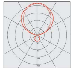
Epur 3 Microperforé 3 x 36 watt
