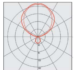
Epur 3 Microperforé 3 x 55 watt
