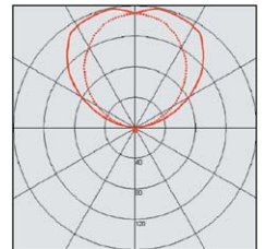
Epur 2 Verre 3 x 55 watt
