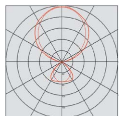
Epur 200-2 2xTL5 35watt
