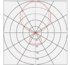
Epur 1 Defilement 3 x 36 watt
